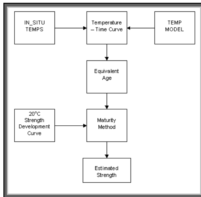
Figure 3 – Maturity Method flowchart, Sub Chart of Figure 1
