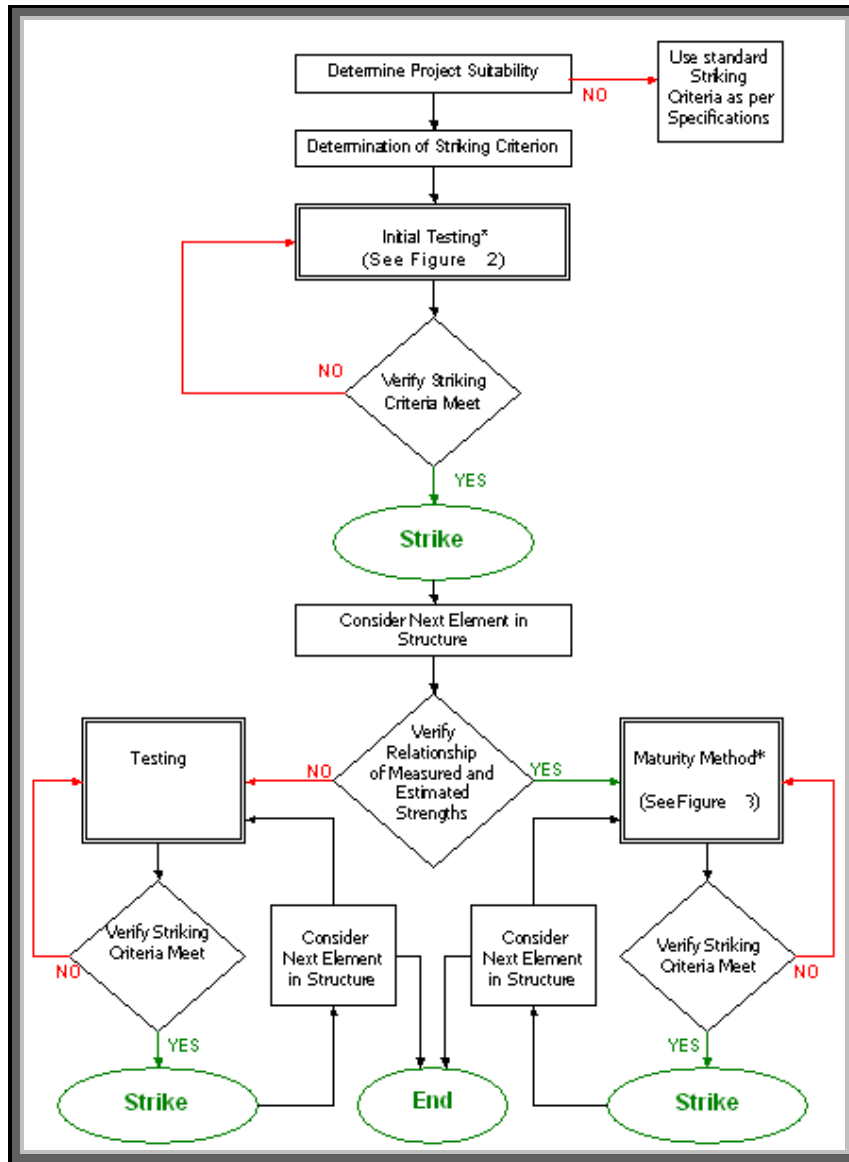
Figure 1 – Decision-Making Flowchart for the Striking of Formwork
