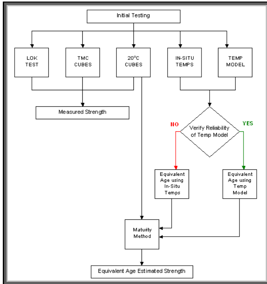
Figure 2 – Initial Testing Programme, Sub Chart of Figure 1
